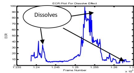
Fig - 12 ECR Graph for Three Consecutive Dissolves
