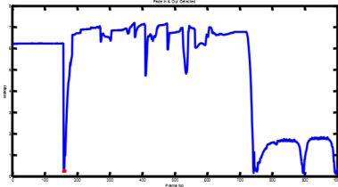
Fig - 7 Entropy Graph for Fade In & Out
