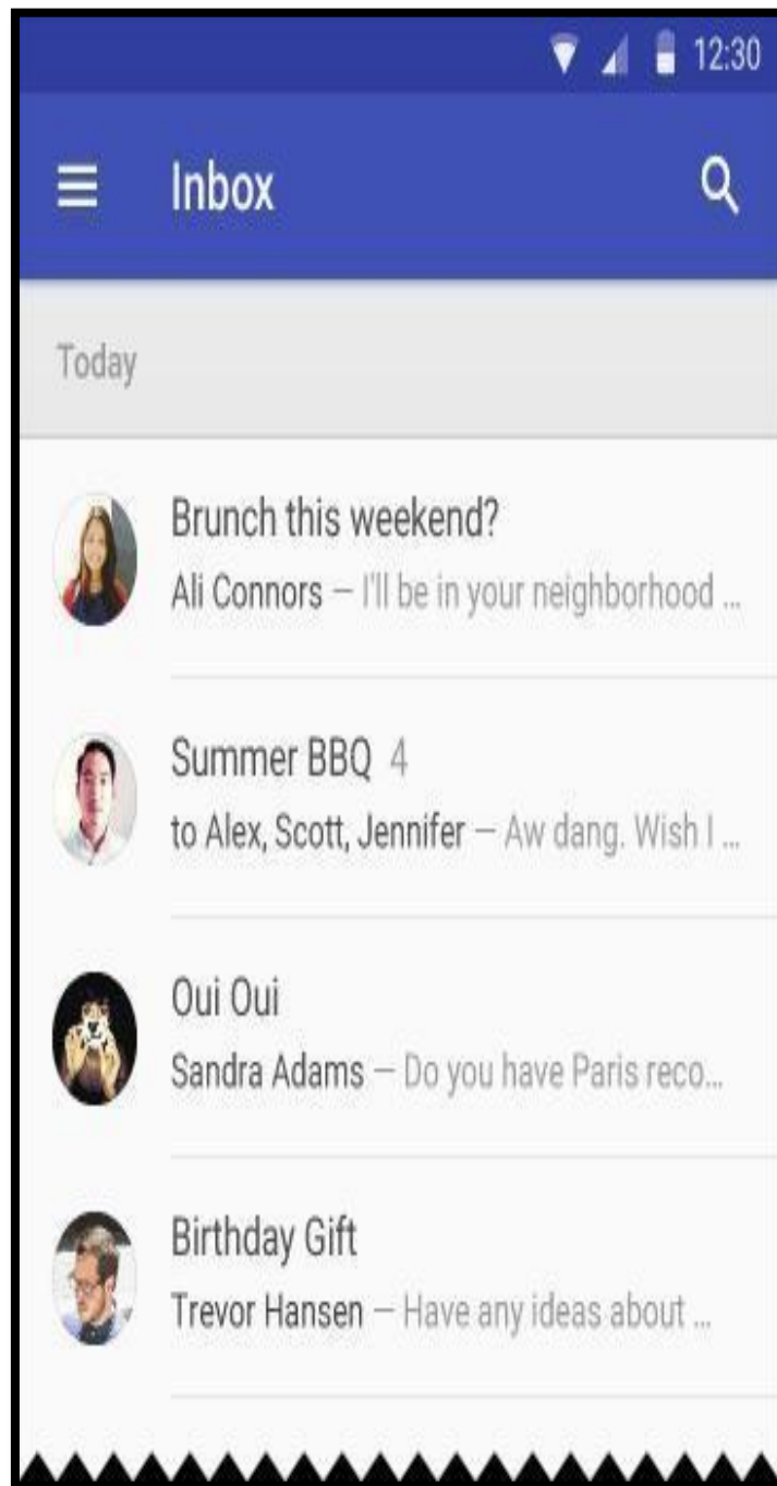
Fig.3.6.2 Home Page
