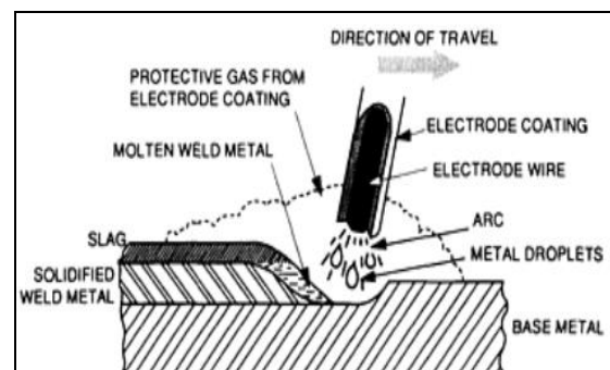
Fig. 1: Arc Welding Setup [1].
