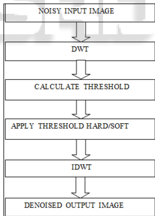
Fig. 3: Wavelet Based Denoising Process
